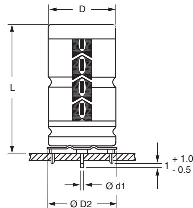
Fig.5 Mounting hole diagramm and outline. Form MR: with mounting ring and pins
