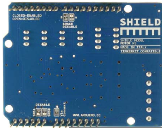
Arduino Motor Shield R3 Back
