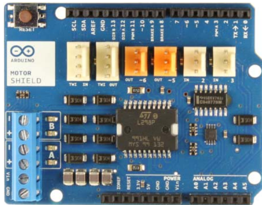
Arduino Motor Shield R3 Front
