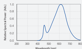
Spectral Power Distribution
