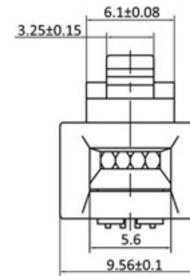
Flat Cable
