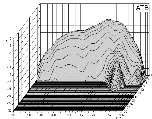
Zerfallsdiagramm TIW 200 XS Messbox 1m / 2.83 V
